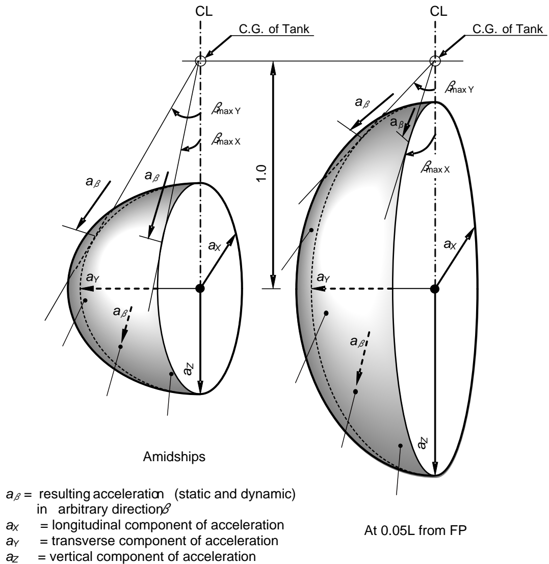
Figure 4.1 – Acceleration ellipsoid
