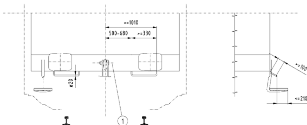
Figure 7: Positions of shunter handrails
