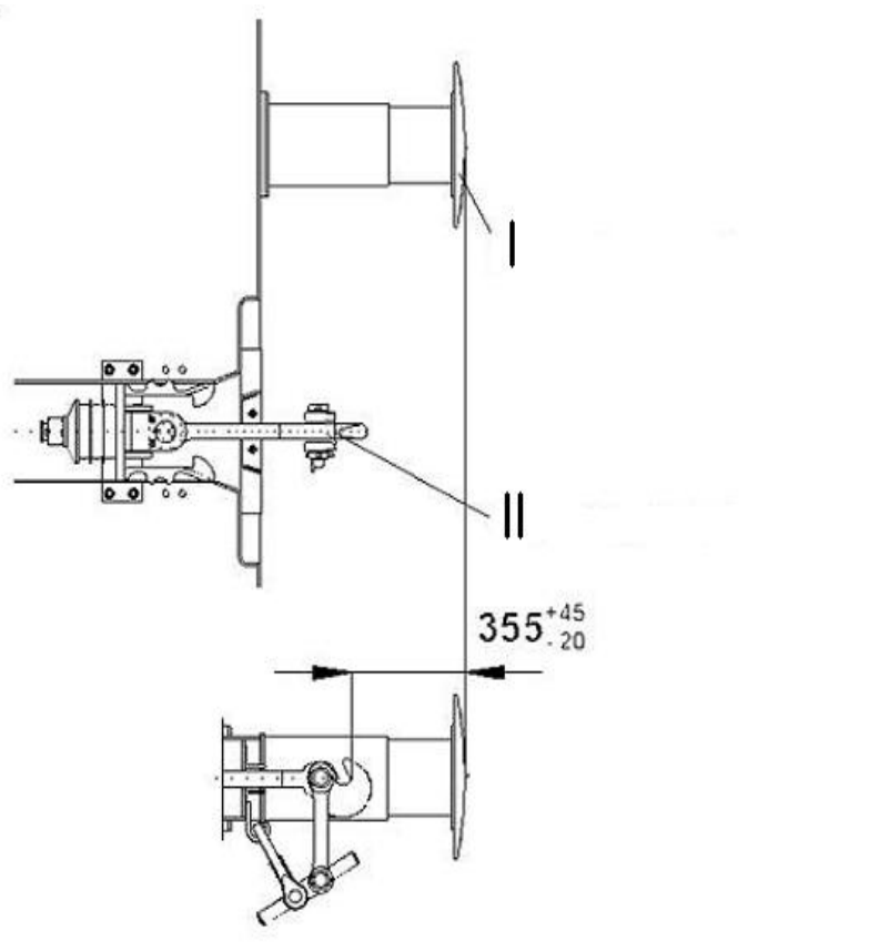
Fig. A1 Draw gear and buffers
